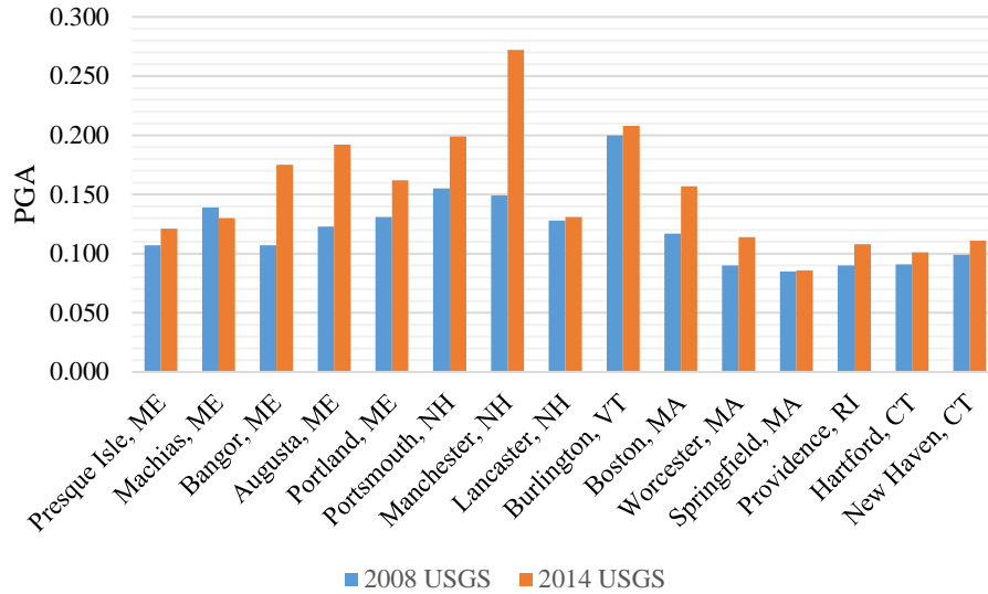
Figure 2 – USGS Hazards Mapping PGA (2% in 50 Years)
