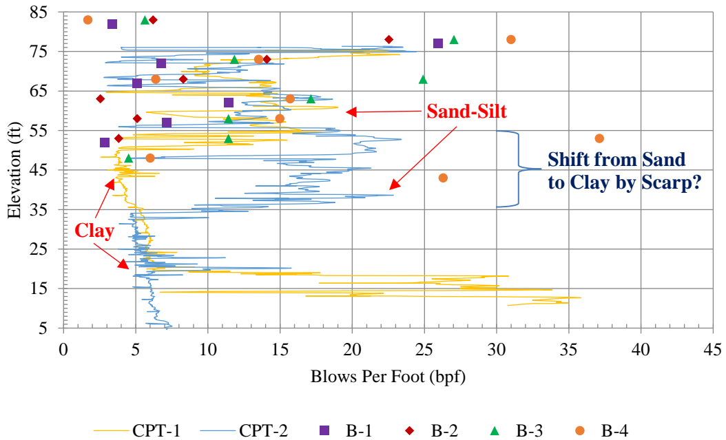
Figure 7 – Standard Penetration Test (SPT N 60 )
