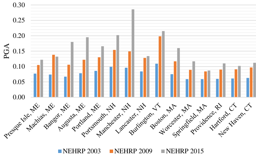
Figure 1a – Peak Ground Acceleration (Site Class B)
