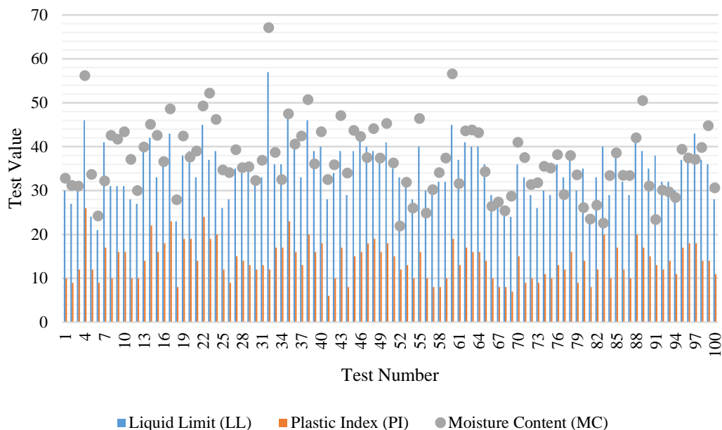
Figure 5 – Atterberg Limit Tests for Presumpscot Formation
