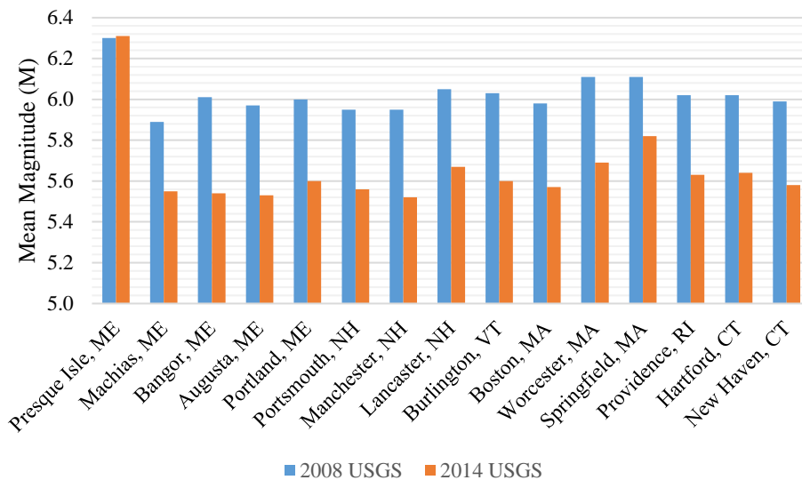
Figure 3 – USGS Hazards Mapping Magnitude (2% in 50 Years)
