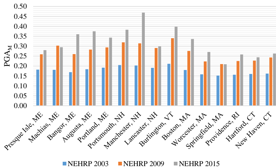
Figure 1b – Peak Ground Acceleration (Site Class E)
