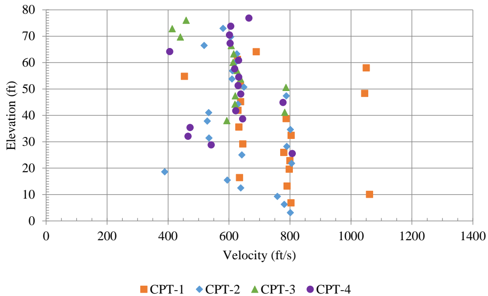
Figure 8 – Shear Wave Velocity (V s )
